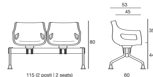
115 (2 posti | 2 seats) 170 (3 posti | 3 seats) 225 (4 posti | 4 seats)
